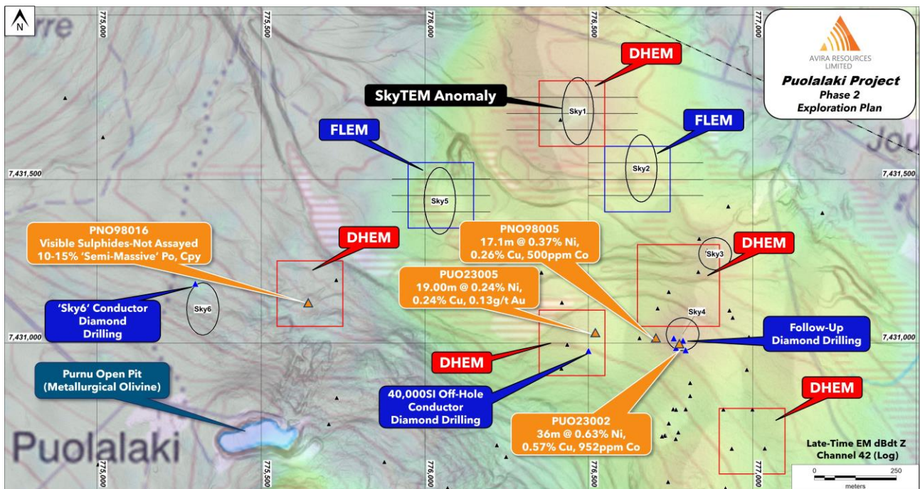
Figure 1: Image showing 'Phase 2' Exploration proposal at the Puolalaki Project. The background image is the Late-Time EM dBdt Z Channel 42 (Log) image, and the black triangles are previously drilled diamond drillholes.
